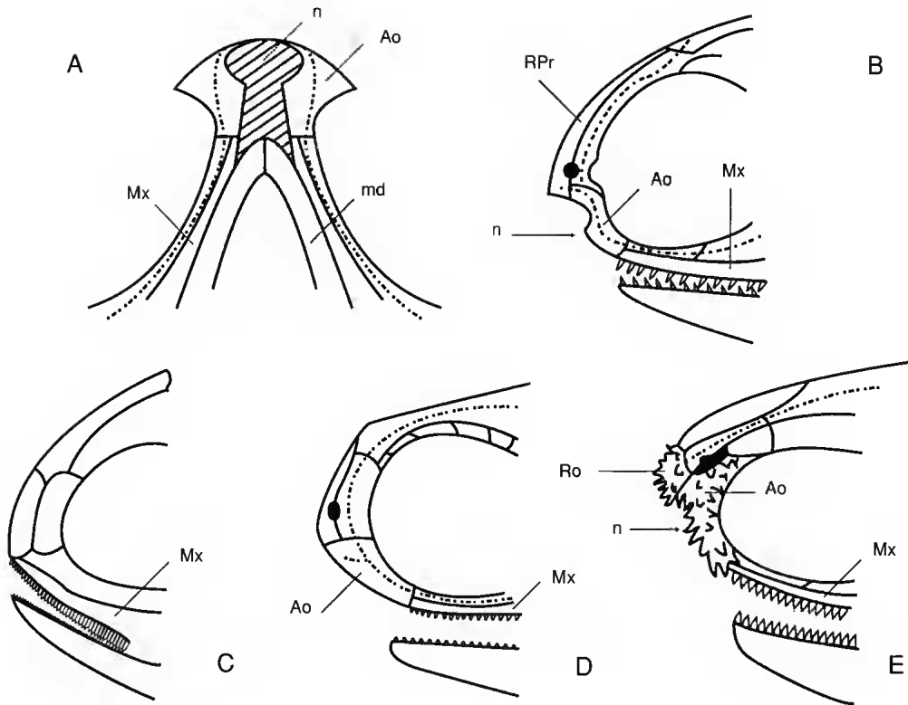
FIG. 2. — Dermal snouts: A , ventral view; B-E , left lateral view. A, B , Rhadinichthyid from Bear Gulch (after Lund & Poplin in prep.); C , Aeduella (after Heyler 1969, fig. 92); D , Palaeoniscus freieslebeni (after Aldinger 1937, fig. 25B); E , Cionichthys greeni (after Schaeffer 1967, fig. 7). Ao , antorbital; Mx , maxillary; md , mandible; n , notch; Ro , rostral; RPr , rostro-postrostral.
